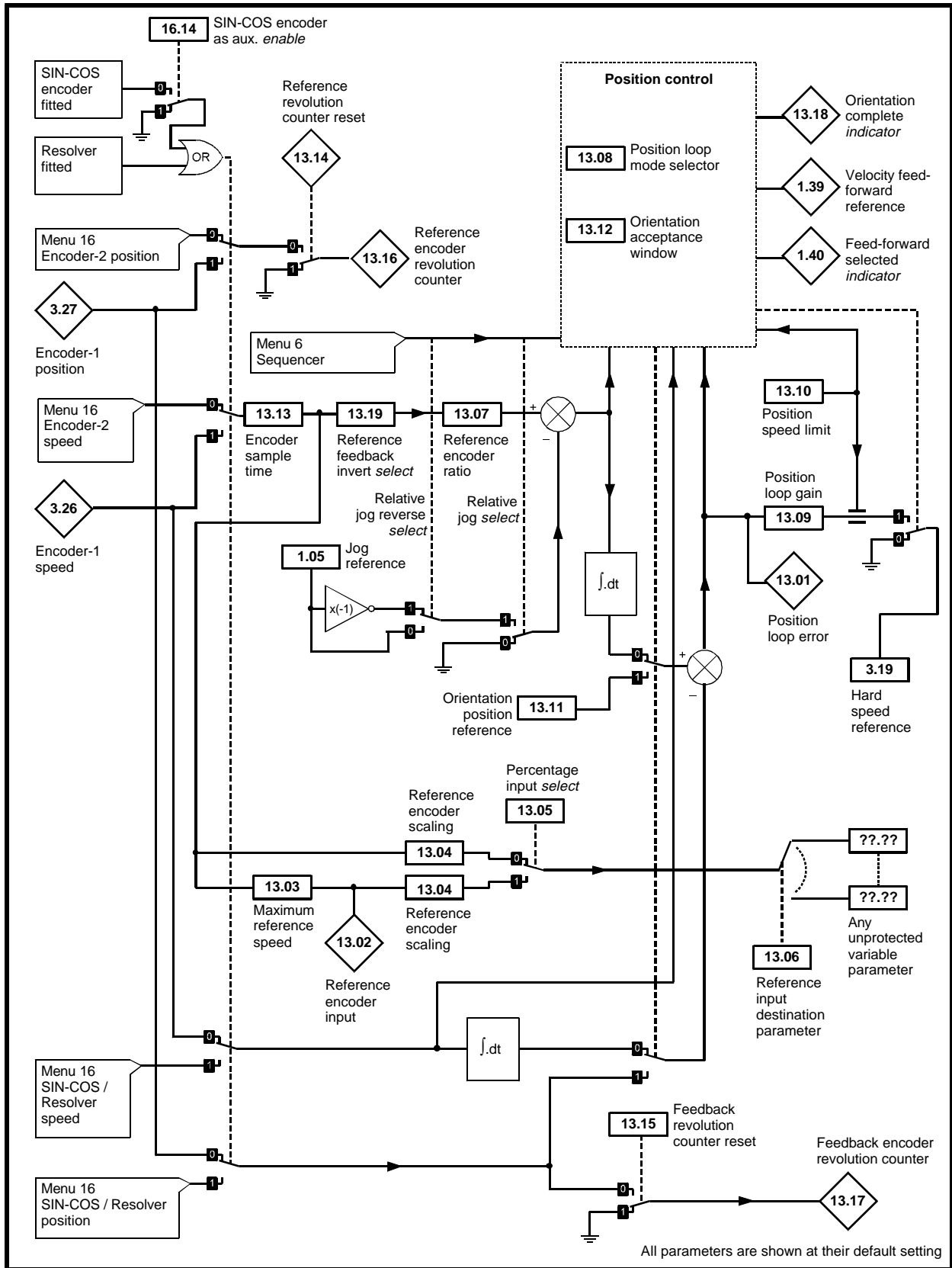
Menu 13 Closed-loop logic diagram
