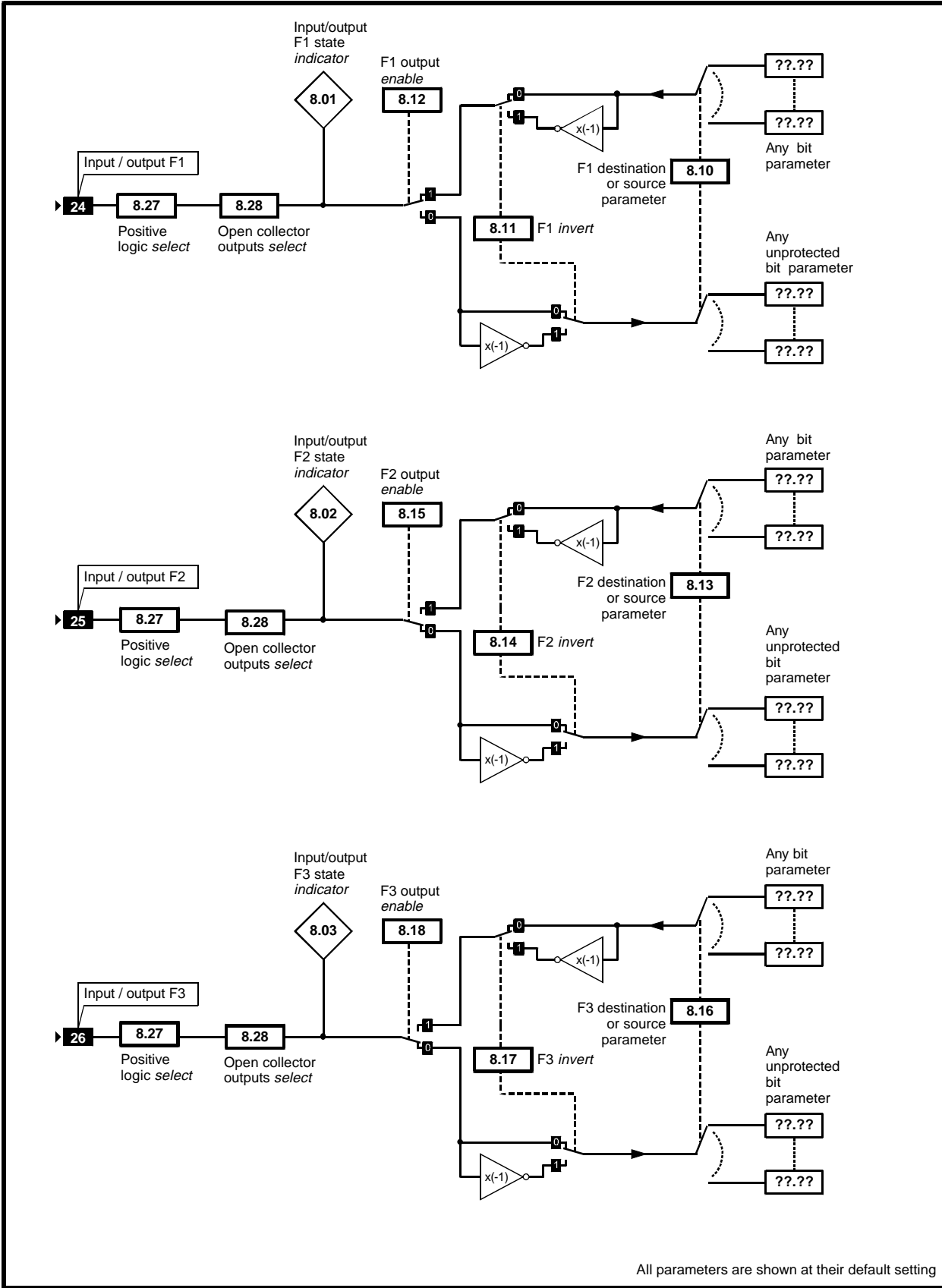
Menu 8 logic diagram
