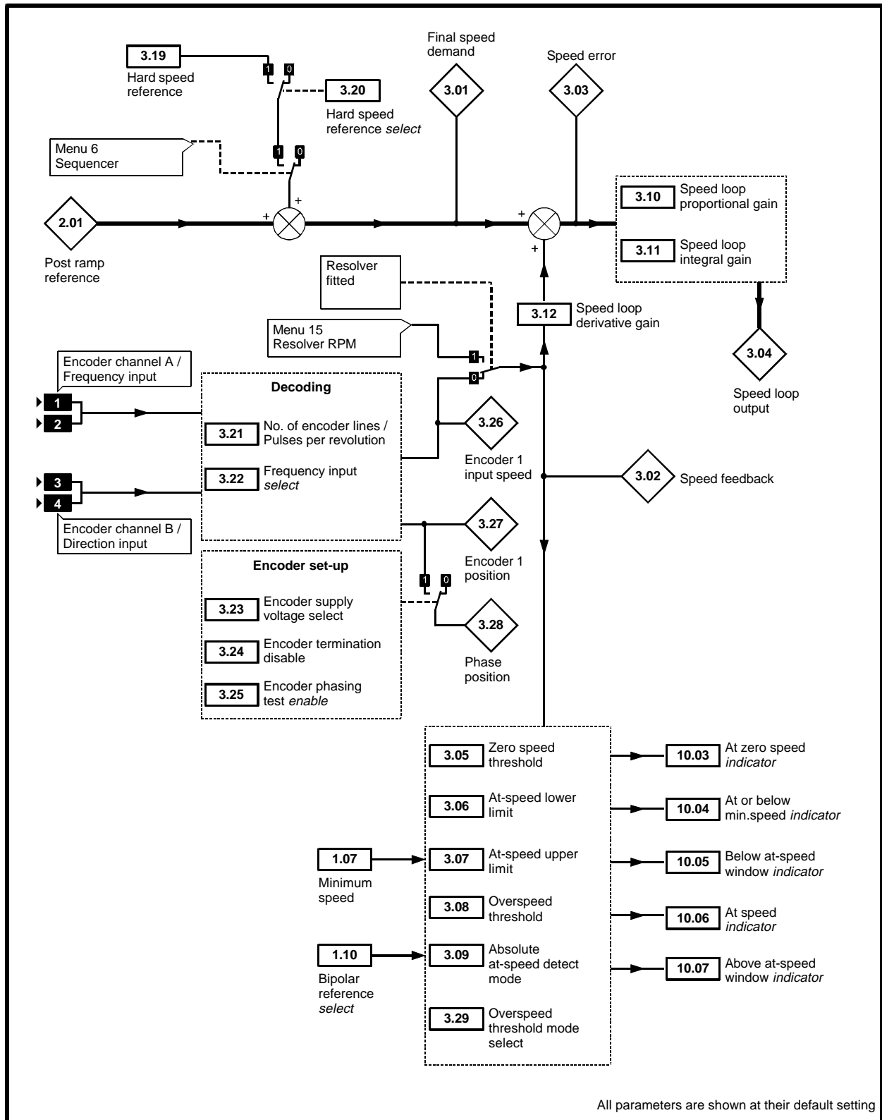
Menu 3 Closed-loop logic diagram
